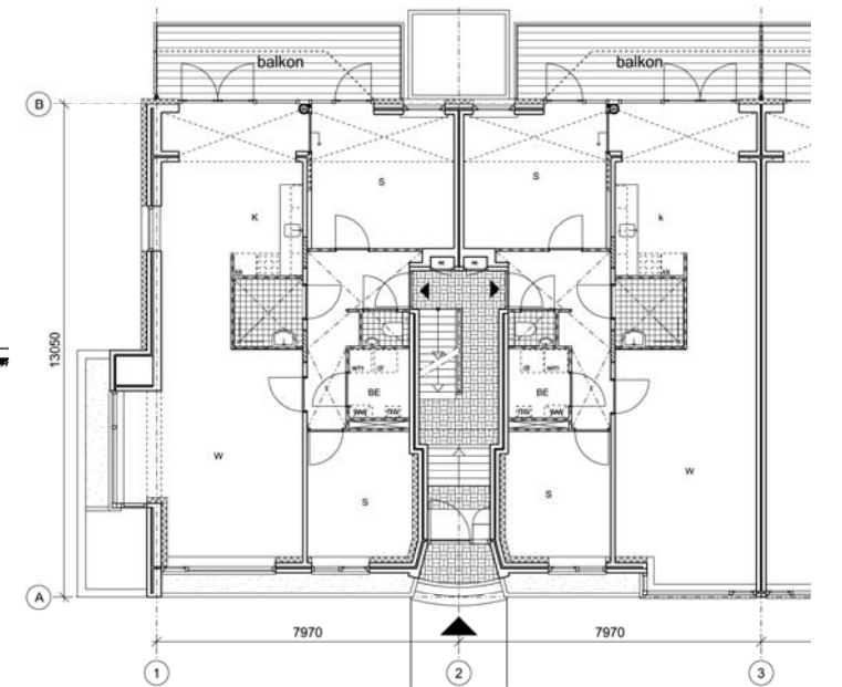
bel-etage
